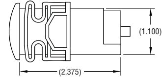
Panel Cutout 2-51/64" x 1-9/64" (71 x 29 mm)
